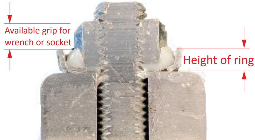
nut with Dubo Toothed Collar Ring
